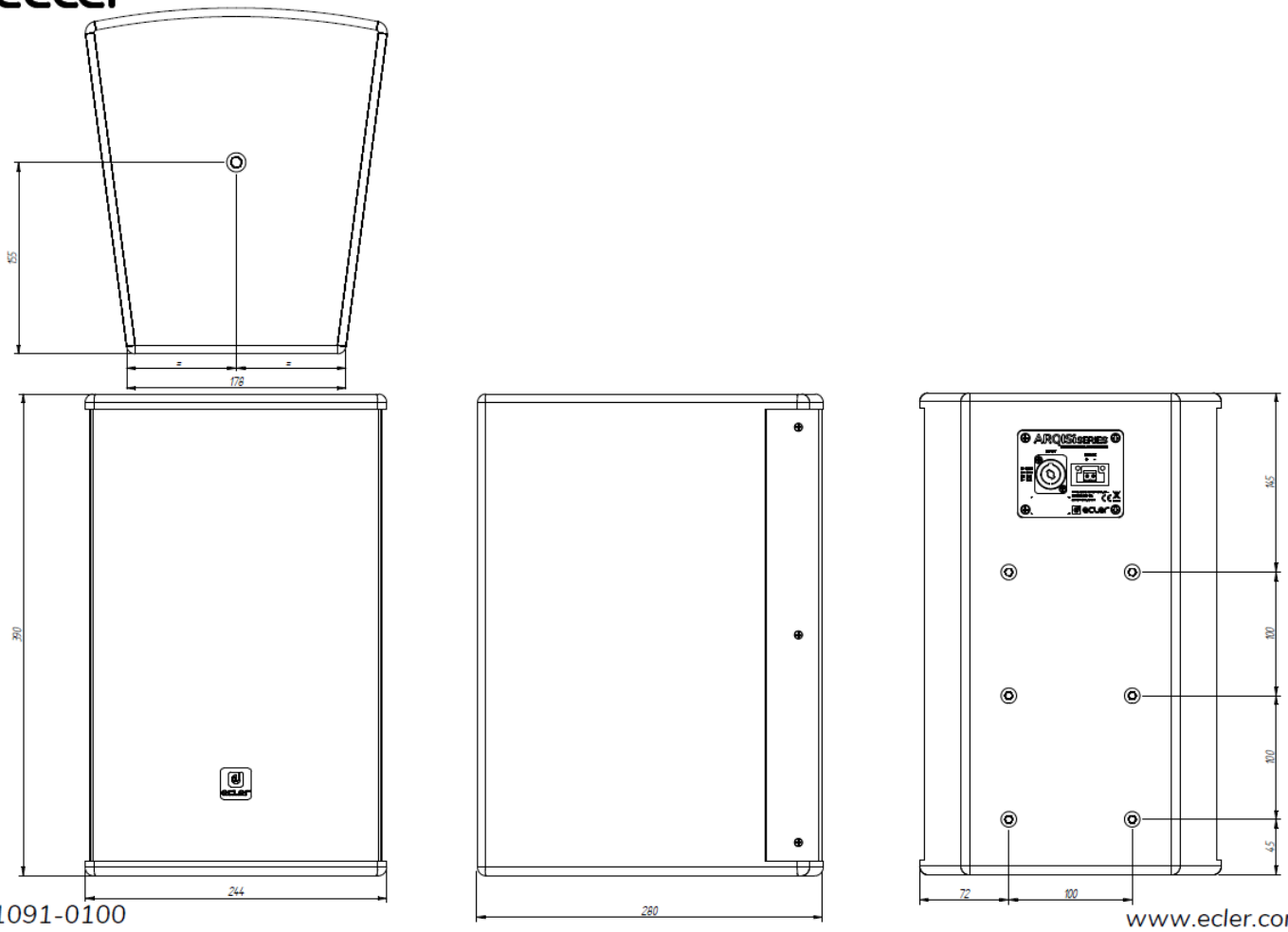
Ecler ARQIS108i Mechanical Diagram
